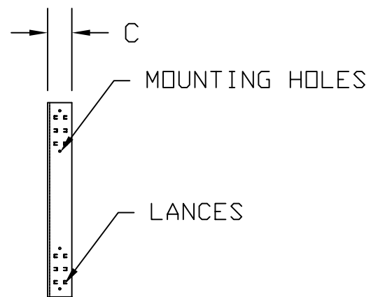
RIGHT-SIDE VIEW
